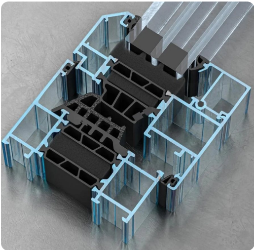
Cross-section
