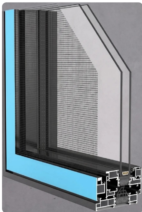
Cross-section
