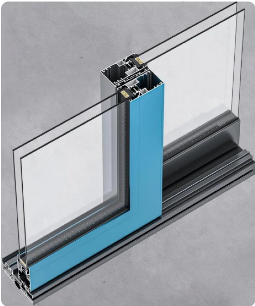
Cross-section
